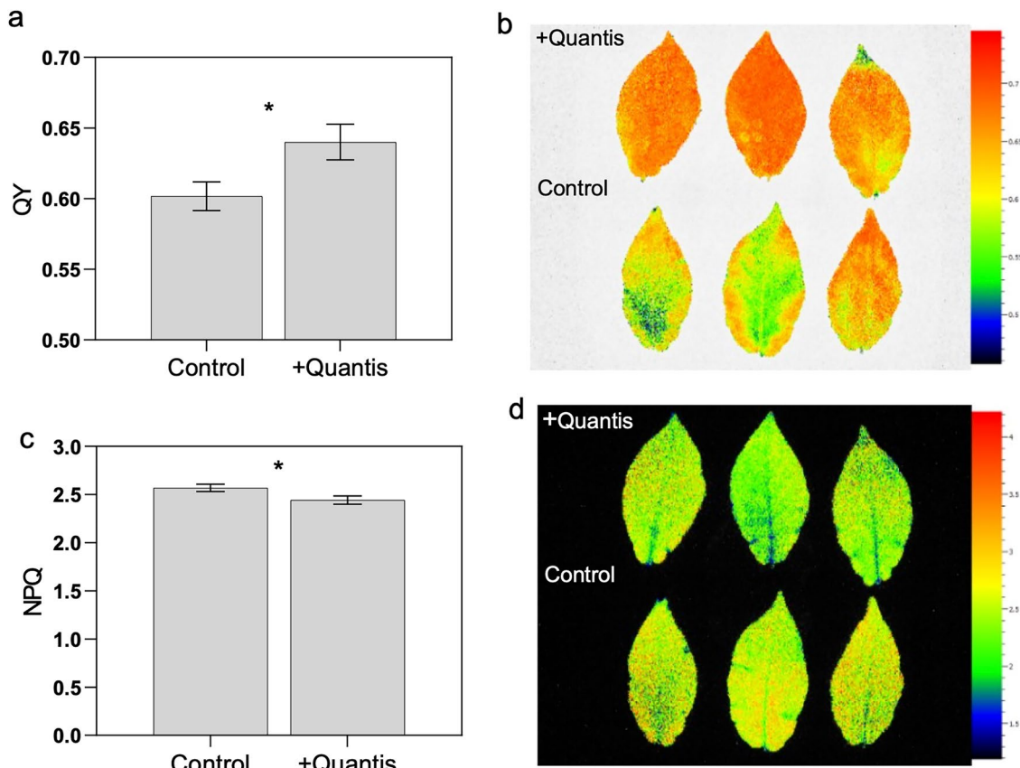
Fig. 3 Chlorophyll fluorescence of Quantis TM -treated and untreated (water-control) detached fully expanded terminal potato (cv. Maris Piper) leaves. a, b Quantum yield (QY), (c,d) non-photochemical quenching (NPQ) measured at 7 days post-application using a closed 800C FluorCam imaging fluorometer (PSI, Czech Republic). Data represent mean \pm SEM of seven biological replicates per treatment with two experimental replicates. Asterisk indicates significant difference according to Student's t test, p < 0.05
